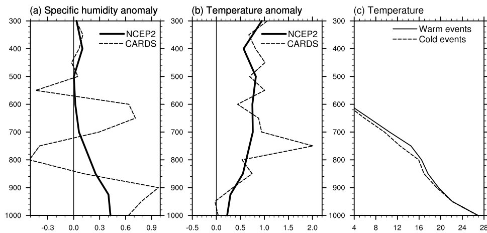
Figure 4. Vertical profiles of (a) specific humidity anomaly and (b) temperature anomaly based on NCEP2 averaged over the southern tropical Atlantic ( 40^{\circ}\text{W} – 0^{\circ} , 0 – 10^{\circ}\text{S} , solid lines) and CARDs ( 8^{\circ}\text{S} , 14^{\circ}\text{W} , dashed lines) in the FMA period. (c) Vertical temperature profiles during the ENSO warm and cold events based on CARDs are plotted by solid and dashed lines, respectively.
