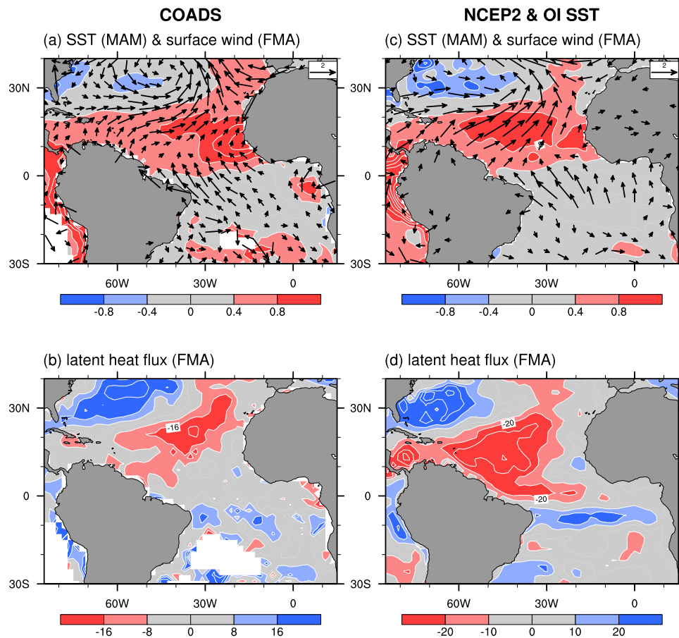
Figure 1. Composite difference maps of (a, c) SSTAs (contour, ^{\circ}\text{C} ) during the MAM period and surface wind anomalies (vector, \text{m s}^{-1} ) during the FMA period and (b, d) latent heat flux anomalies (contour, \text{W m}^{-2} ) during the FMA period between the ENSO warm and cold events. Left (right) plots are based on COADS (NCEP2 and OI SST). Zero contours are omitted. Warm (cold) colors in bottom plots indicate heat gain (loss) from the ocean.
