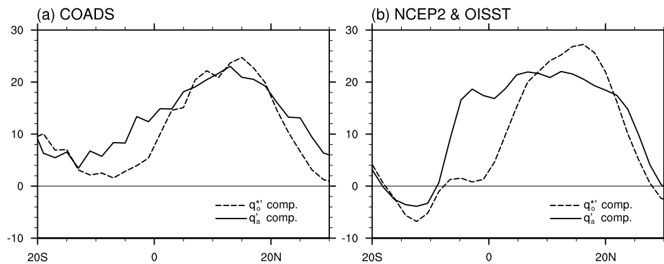
Figure 3. Latitude distributions of contributions from saturation specific humidity at the sea surface ( q_o^{*} , dashed lines) and from air specific humidity anomaly ( q_a' , solid lines) to latent heat flux anomalies based on (a) COADS and (b) NCEP2 and OISST. These anomaly components are zonally averaged over the tropical Atlantic ( 70^\circ\text{W} – 0^\circ ). Units are \text{W m}^{-2} . Difference between the q_o^{*} and q_a' components is identical to the \Delta q' component.
