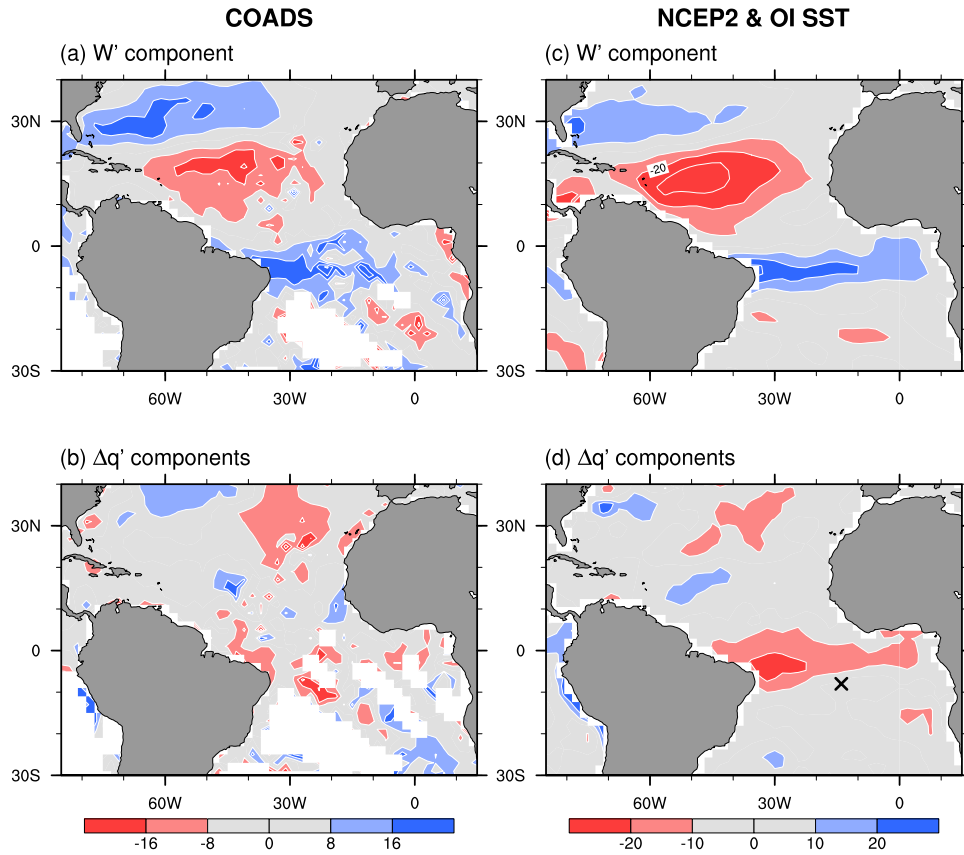
Figure 2. Same as Figures 1b and 1d but for contributions from (a, c) wind speed anomalies ( W' ) and (b, d) air-sea difference in specific humidity ( \Delta q' ) to latent heat flux anomalies. Cross in Figure 1d indicates the station at Ascension Island.
