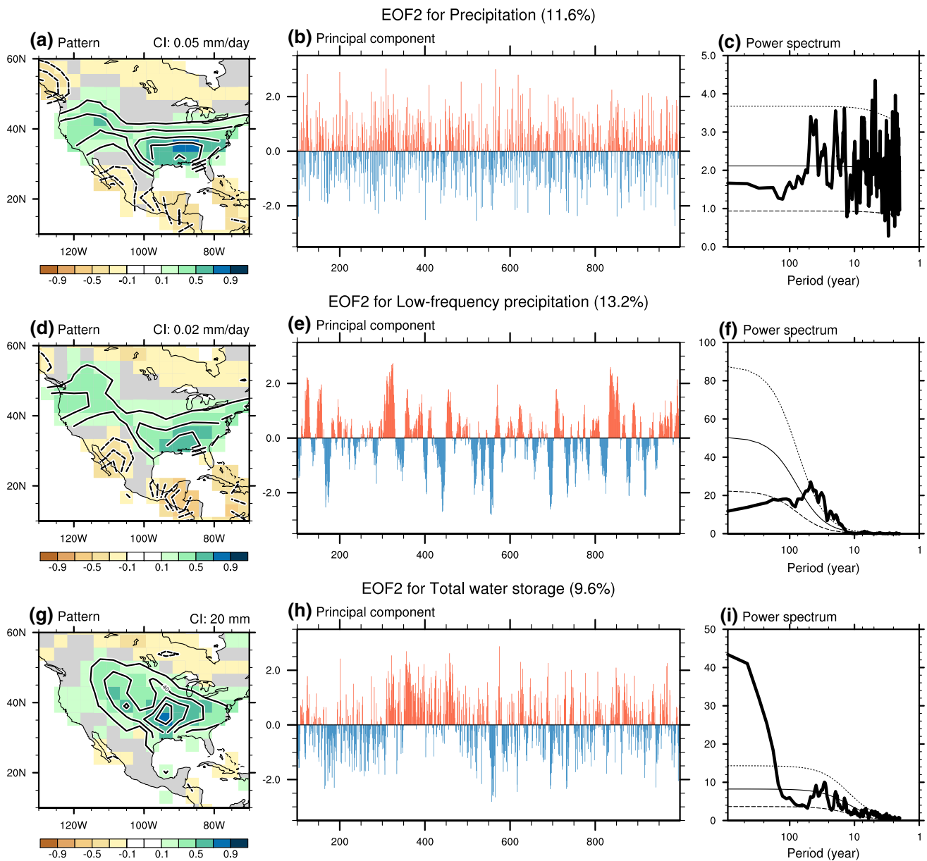
Fig. 7 Same as Fig. 4, but for the second EOF mode
